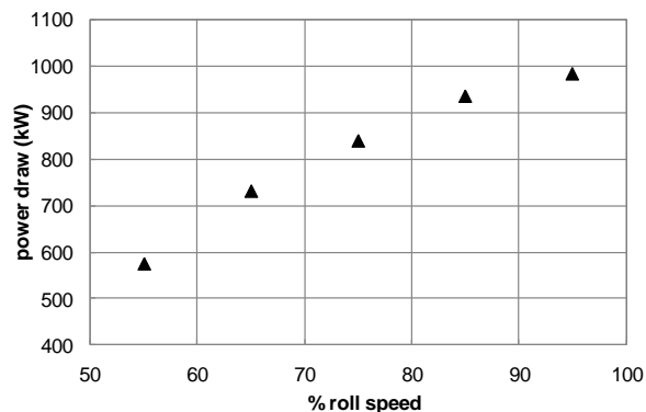
Figure 1. Rolls'speed vs. power draw
